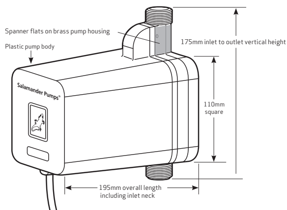
Figure 1: Spanner flats to hold the CombiBoost during installation
