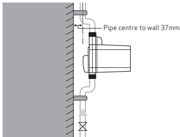
Figure 4: Modified pipe work for clearance
